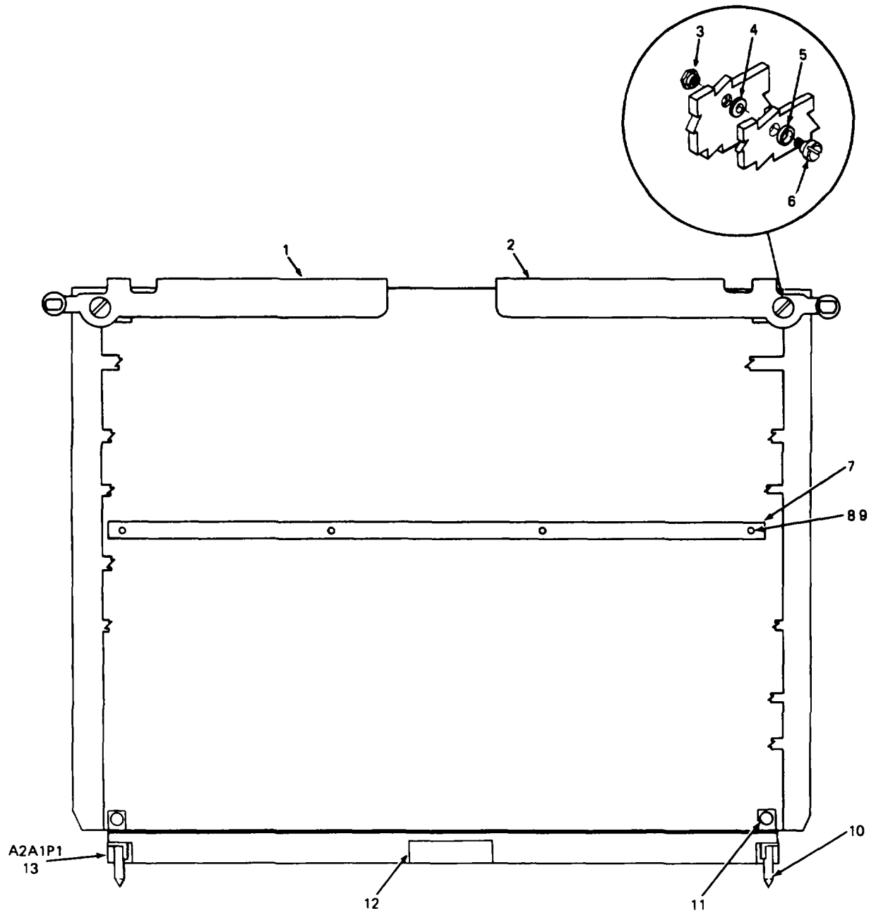
FIGURE 42. INTERFACE ADAPTER ASSEMBLY
