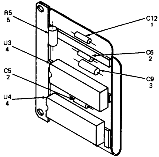
FIGURE 36. UNIBUS TERMINATOR FLEXIBLE WIRING ASSEMBLY A1
