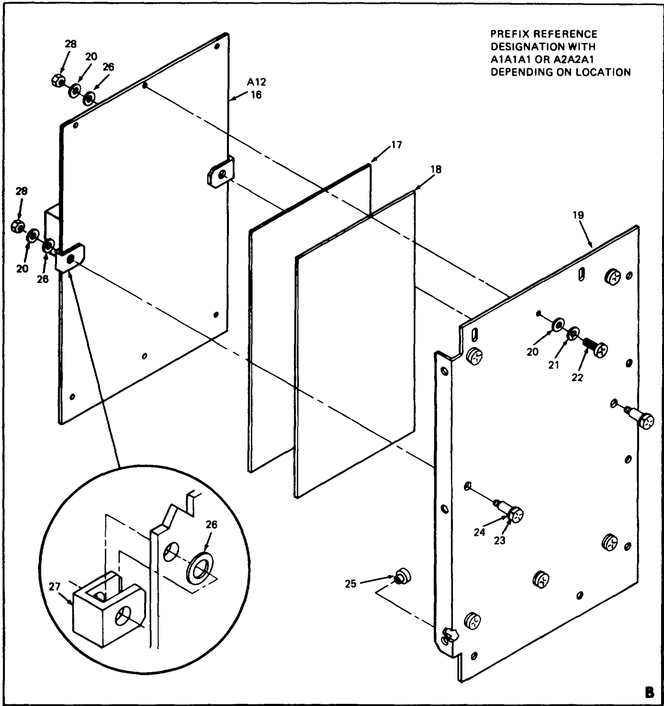
FIGURE 5. 70 AMP POWER SUPPLY (SHEET 3 OF 8)
