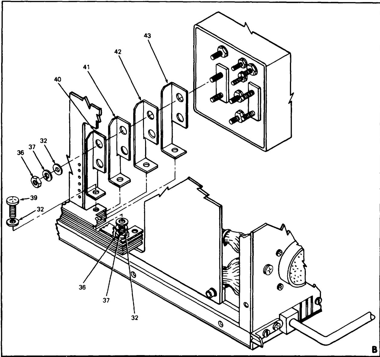
FIGURE 3. HOUSING ASSEMBLY, CPU (SHEET 2 OF 4)
