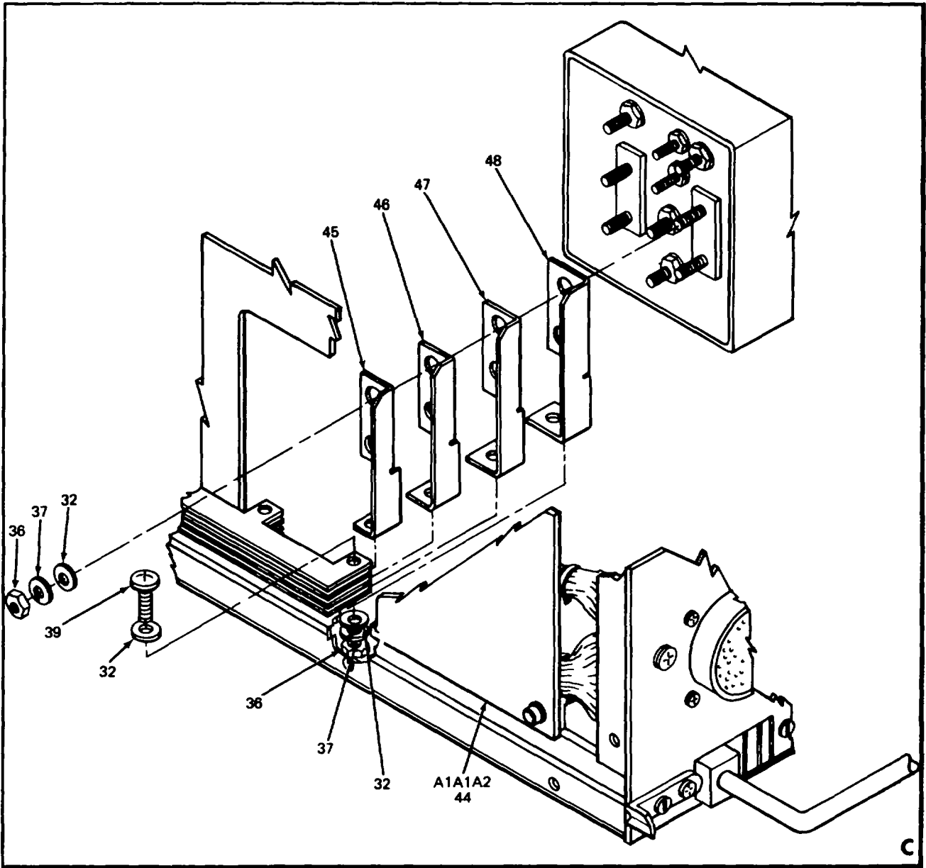
FIGURE 3. HOUSING ASSEMBLY, CPU (SHEET 4 OF 4)
