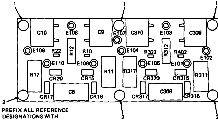
FIGURE 8. SNUBBER COMPONENT BOARD ASSEMBLY
