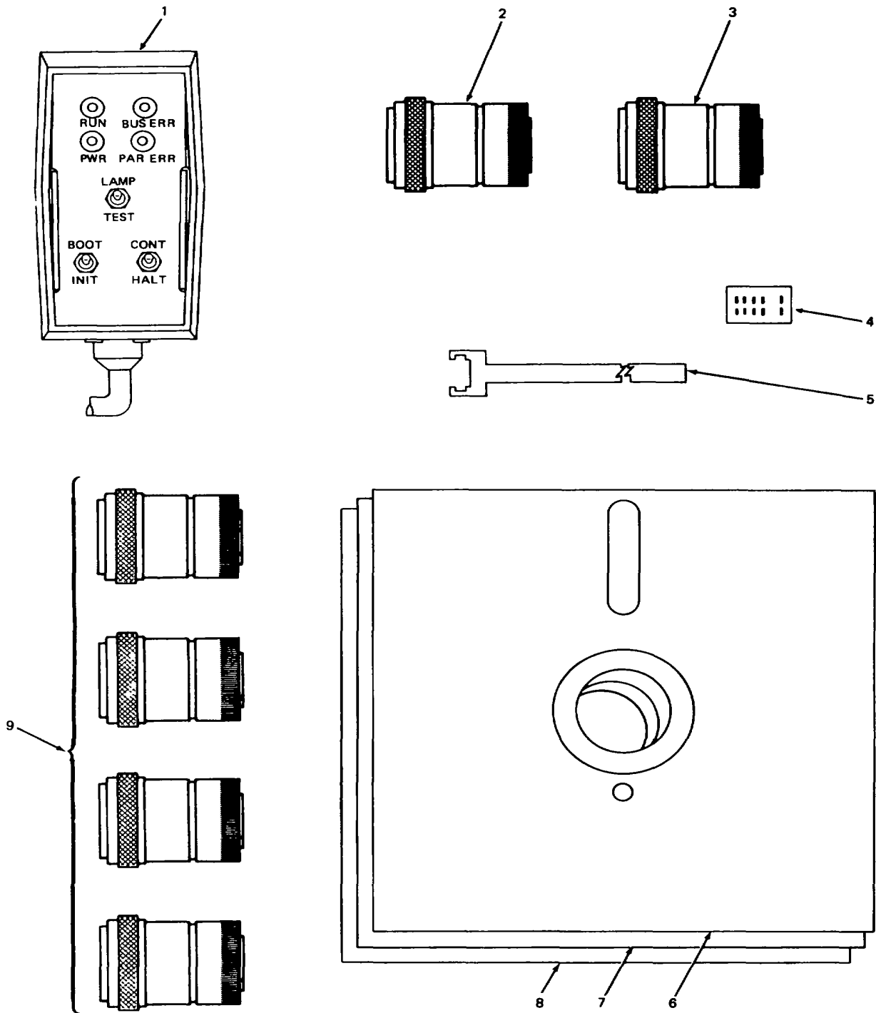
FIGURE 45. SPECIAL TOOLS
