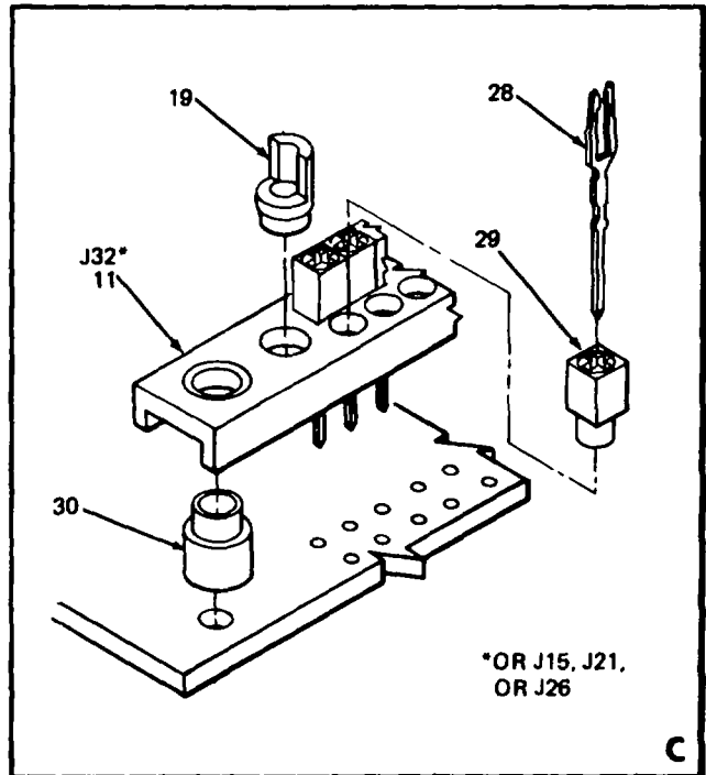
FIGURE 40. GRANDMOTHER BOARD, EXPANDER ASSEMBLY (SHEET 2 OF 3)
