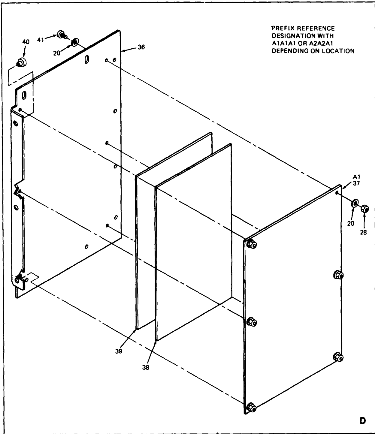
FIGURE 5. 70 AMP POWER SUPPLY (SHEET 5 OF 81)
