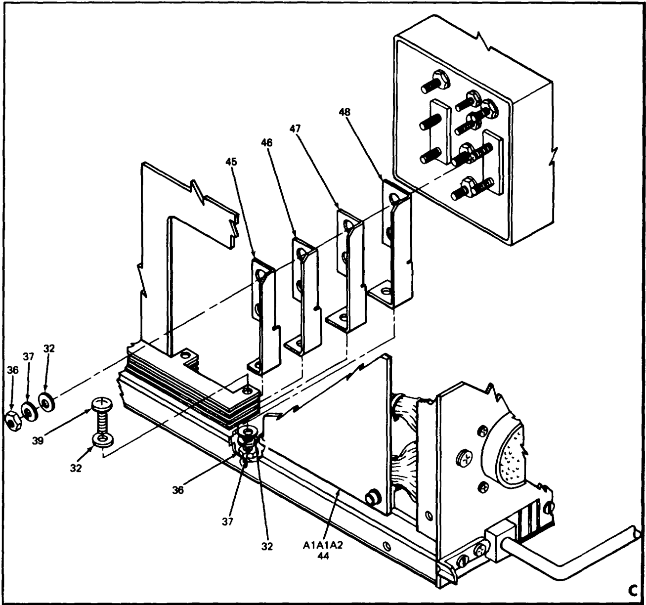
FIGURE 3. HOUSING ASSEMBLY, CPU (SHEET 3 OF 4)
