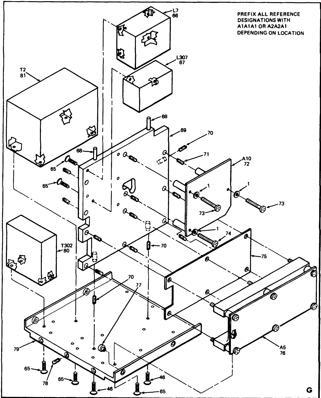
FIGURE 5. 70 AMP POWER SUPPLY (SHEET 8 OF 8)
