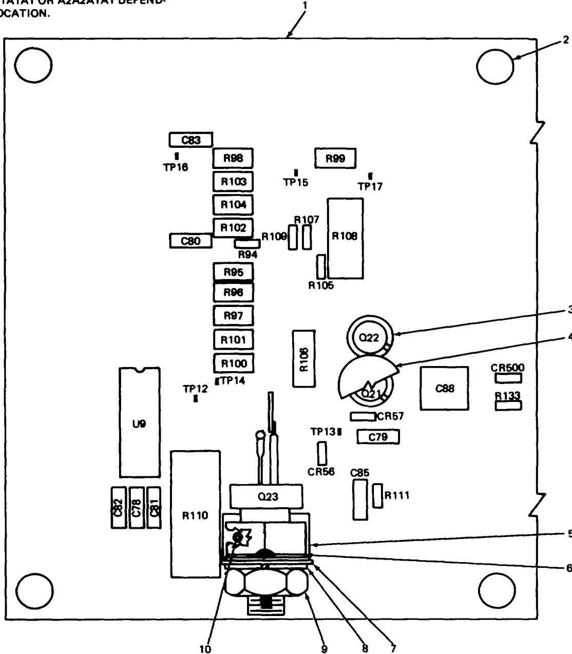
Figure 6. AC DC LO ASSEMBLY (SHEET 1 OF 2)
