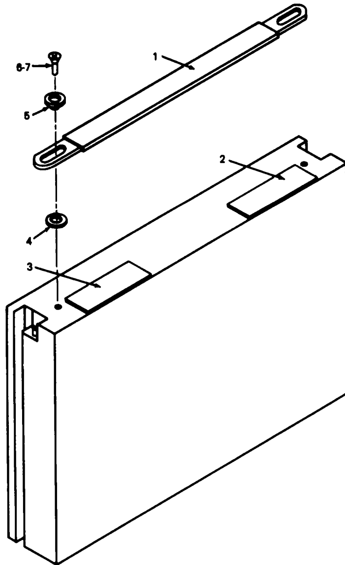
FIGURE 30. 32K WORD CORE MEMORY ASSEMBLY
