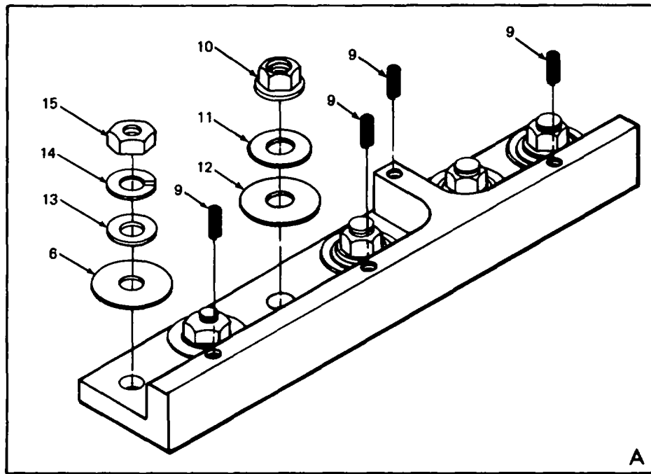
FIGURE 12. OUTPUT RECTIFIER HEATSINK ASSEMBLY
