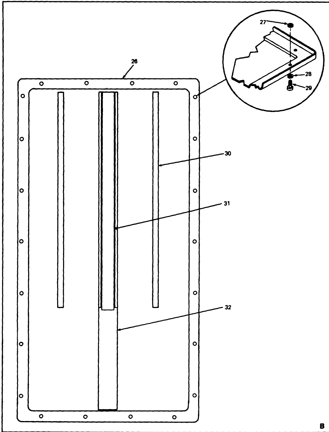
FIGURE 2. COMPUTER MINI (SHEET 2 OF 2)
