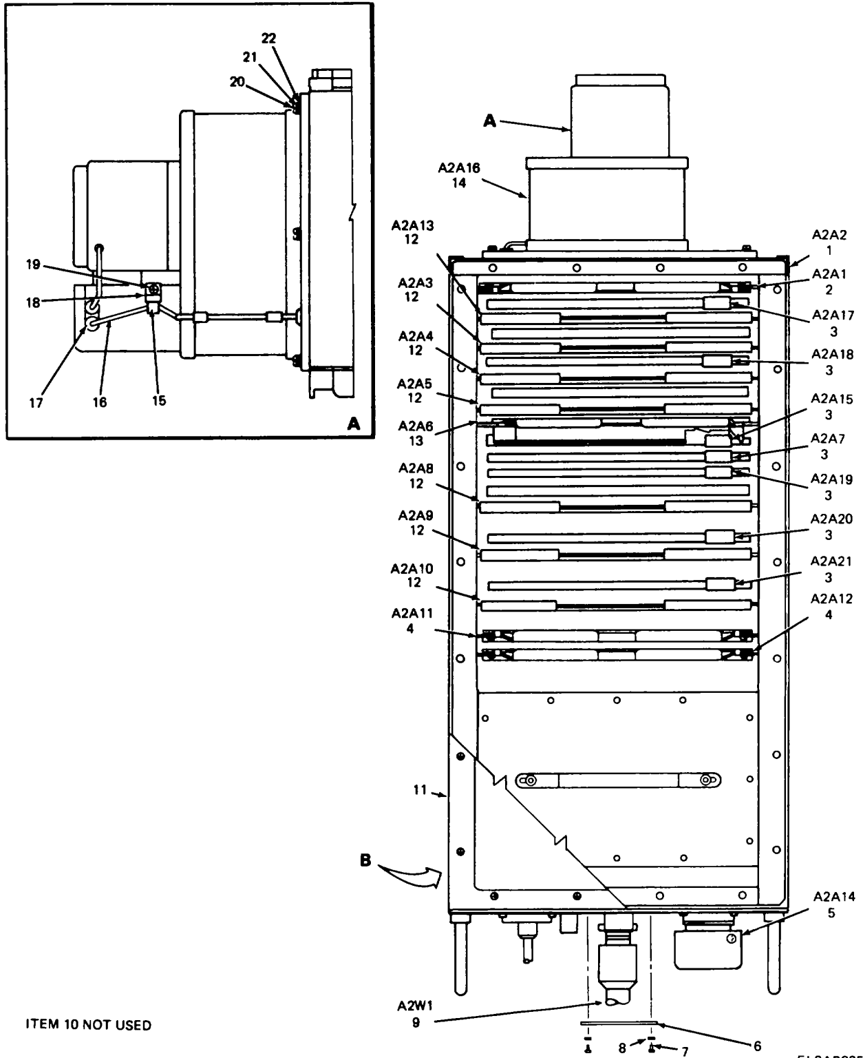
FIGURE 34. COMPUTER, DIGITAL MINI I/O EXPANDER (SHEET 1 OF 2)
