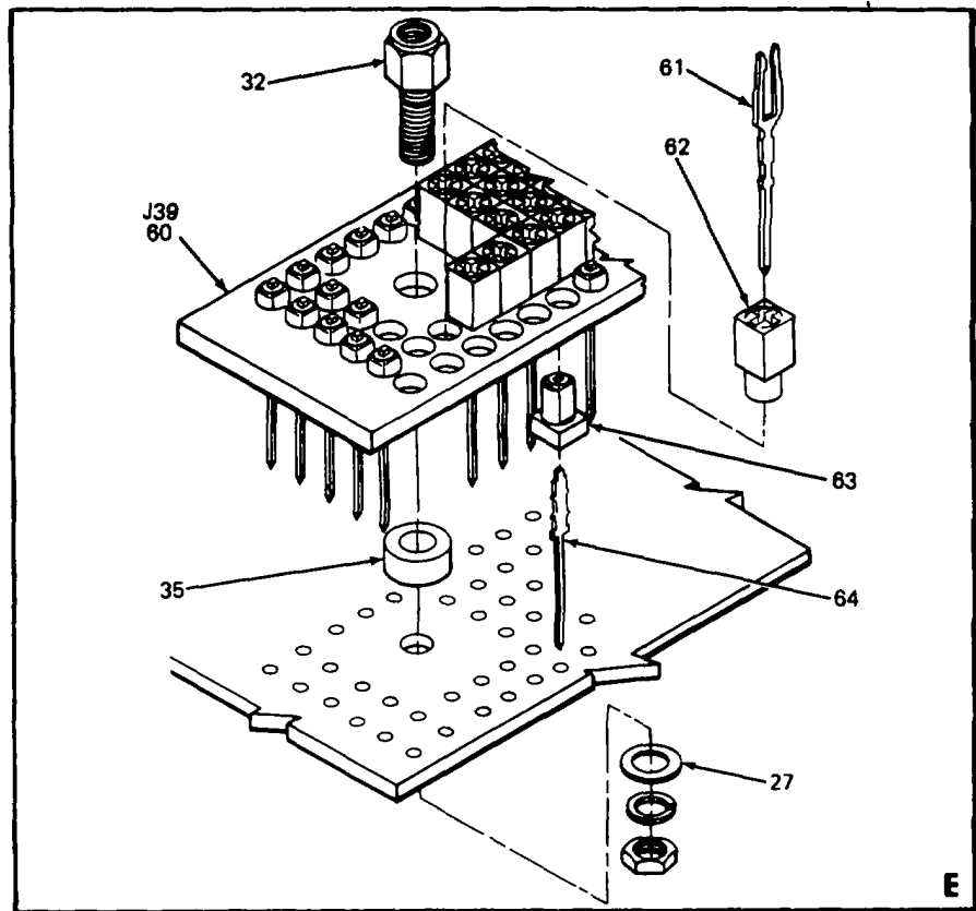
FIGURE 40. GRANDMOTHER BOARD, EXPANDER ASSEMBLY (SHEET 3 OF 3)
