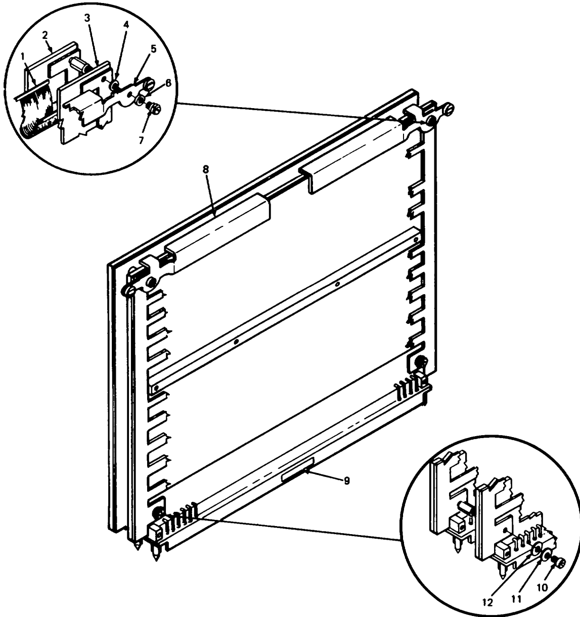
FIGURE 25. CPU CONTROL-SPECIAL
