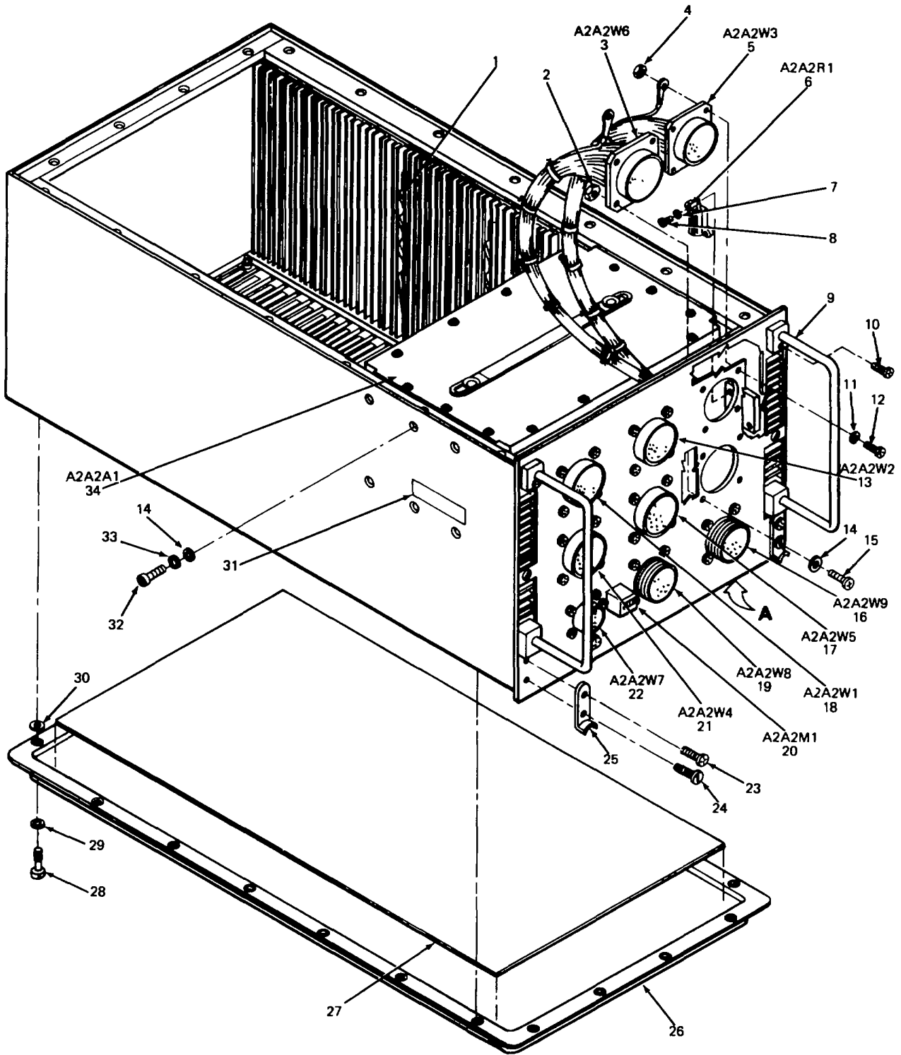
FIGURE 39. HOUSING ASSEMBLY, EXPANDER (SHEET 1 OF 4)
